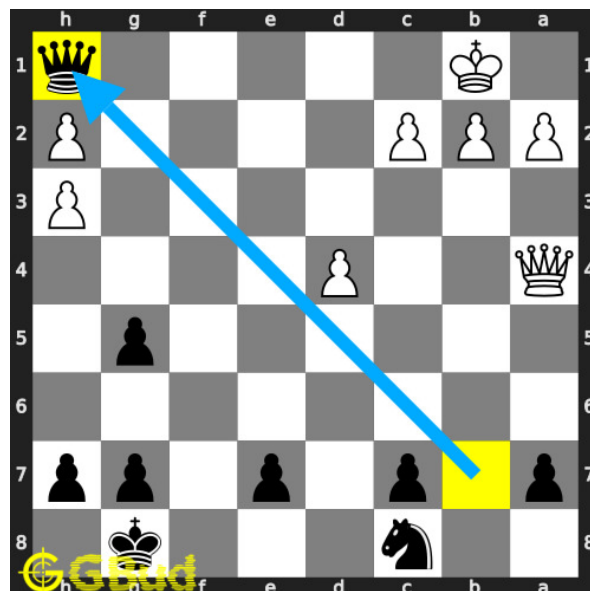
Figure 5: Qxh1#
